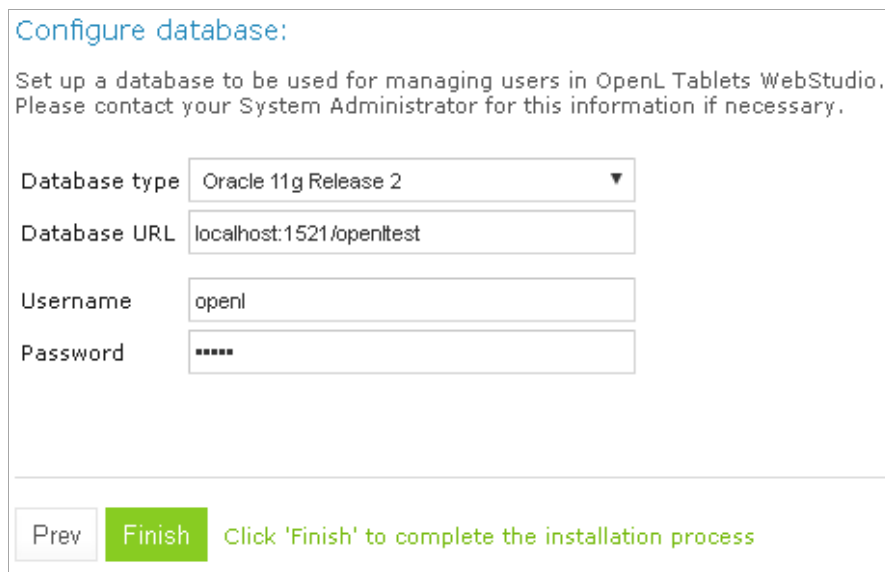
Figure 3: Creating a connection to the Oracle database in the installation wizard
