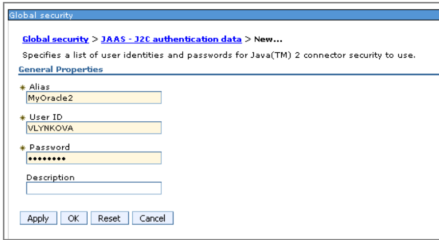
Figure 11: Setting up global security in WebSphere
