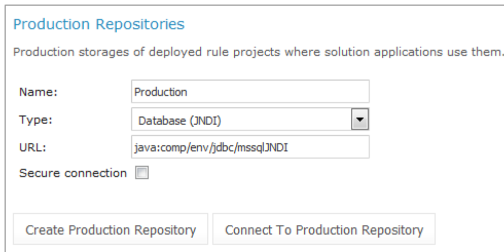
Figure 7: Setting up JNDI connection with installation wizard
